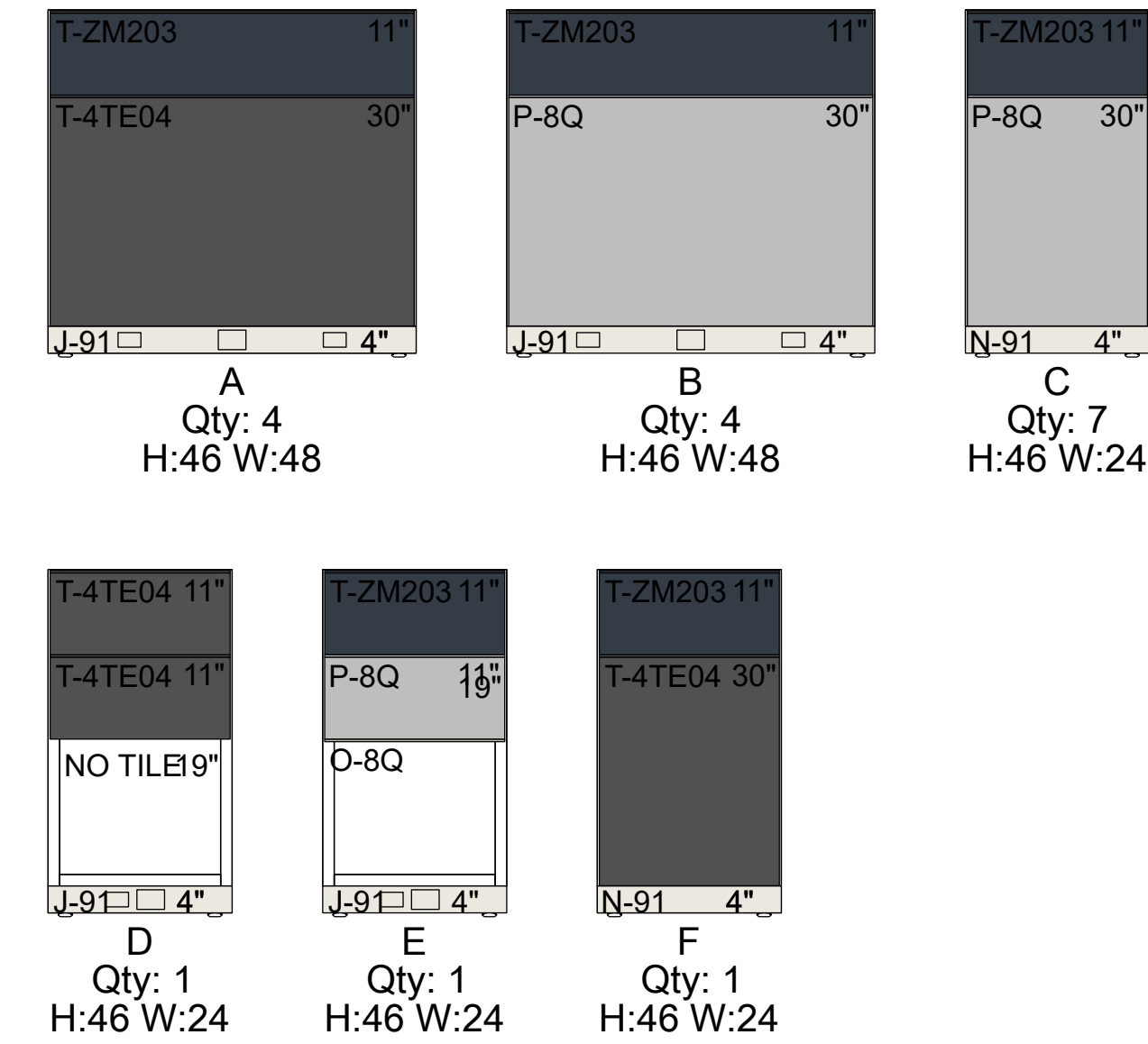
Frame Side Type Elevation - C003
