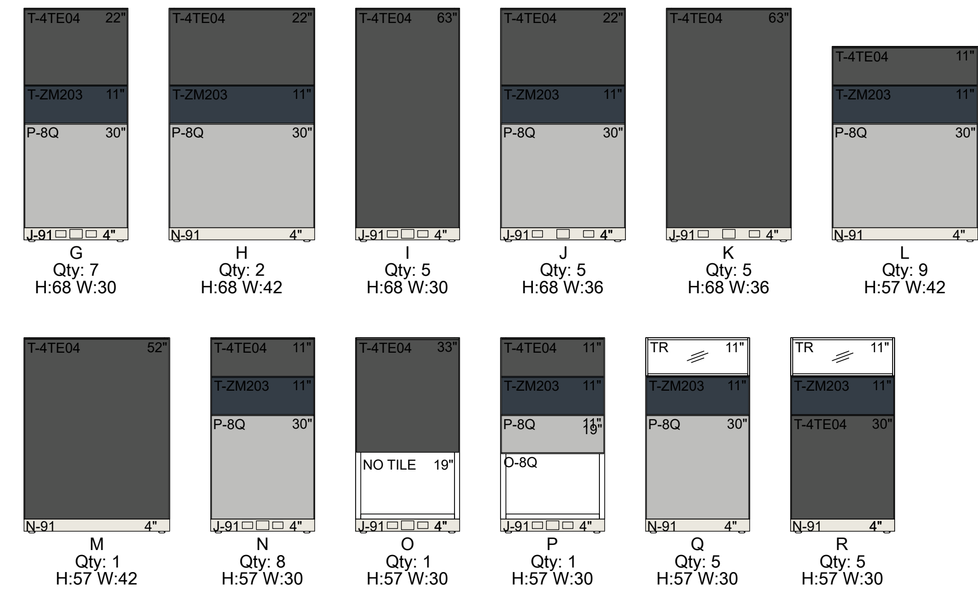
Frame Side Type Elevation - C001
