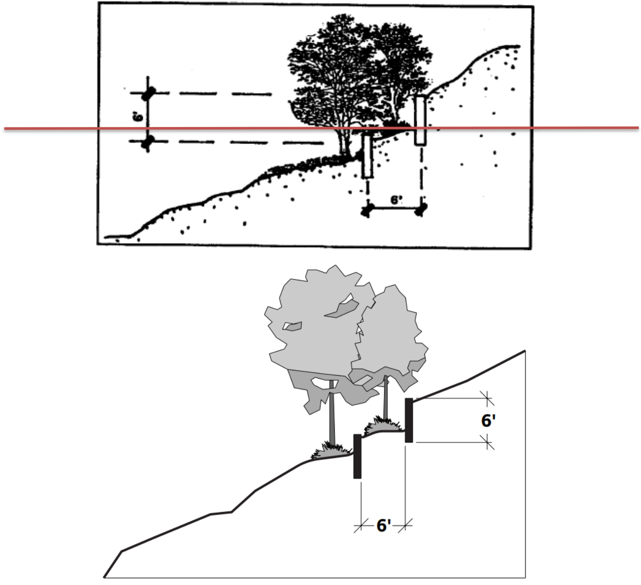
FIGURE 3-716.24-2 HEIGHT OF RETAINING WALLS
