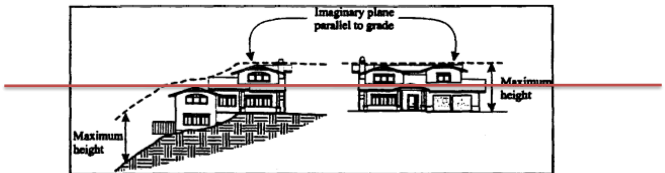
FIGURE 3-1 HEIGHT MEASUREMENT
