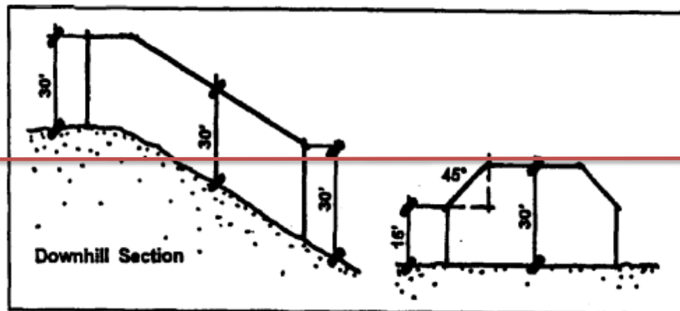
FIGURE 3-4 BUILDING ENVELOPE FOR DOWNHILL LOT
