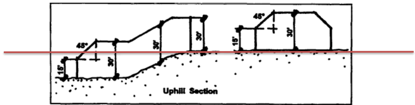
FIGURE 3-5 BUILDING ENVELOPE FOR UPHILL LOT
